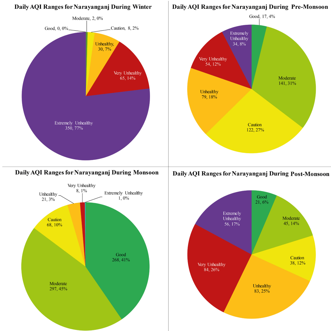
Fig. 6. The ranges of daily AQI for Narayanganj
