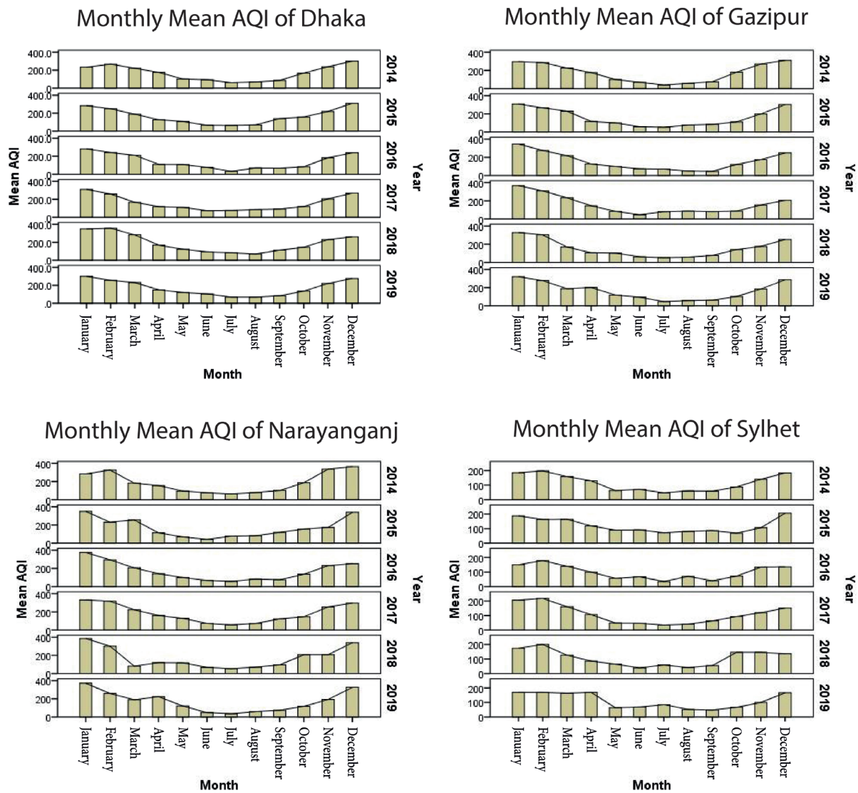
Fig. 8. The monthly mean of AQI in (a) Barisal; (b) Chattogram; (c) Dhaka; (d) Gazipur; (e) Narayanganj; (f) Sylhet stations of CAMS in Bangladesh from 2014 to 2019
