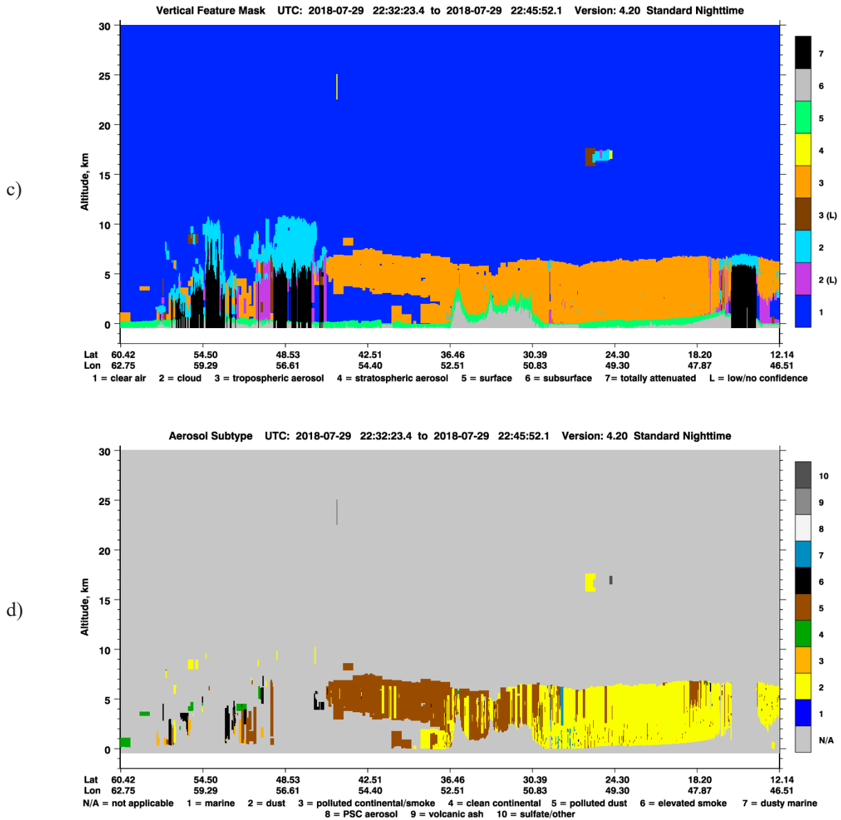
Fig. 6. a) The CALIPSO satellite path, b) total attenuated backscatter, c) vertical feature mask, d) aerosol type at 22:32 to 22:45 UTC on July 29, 2018
