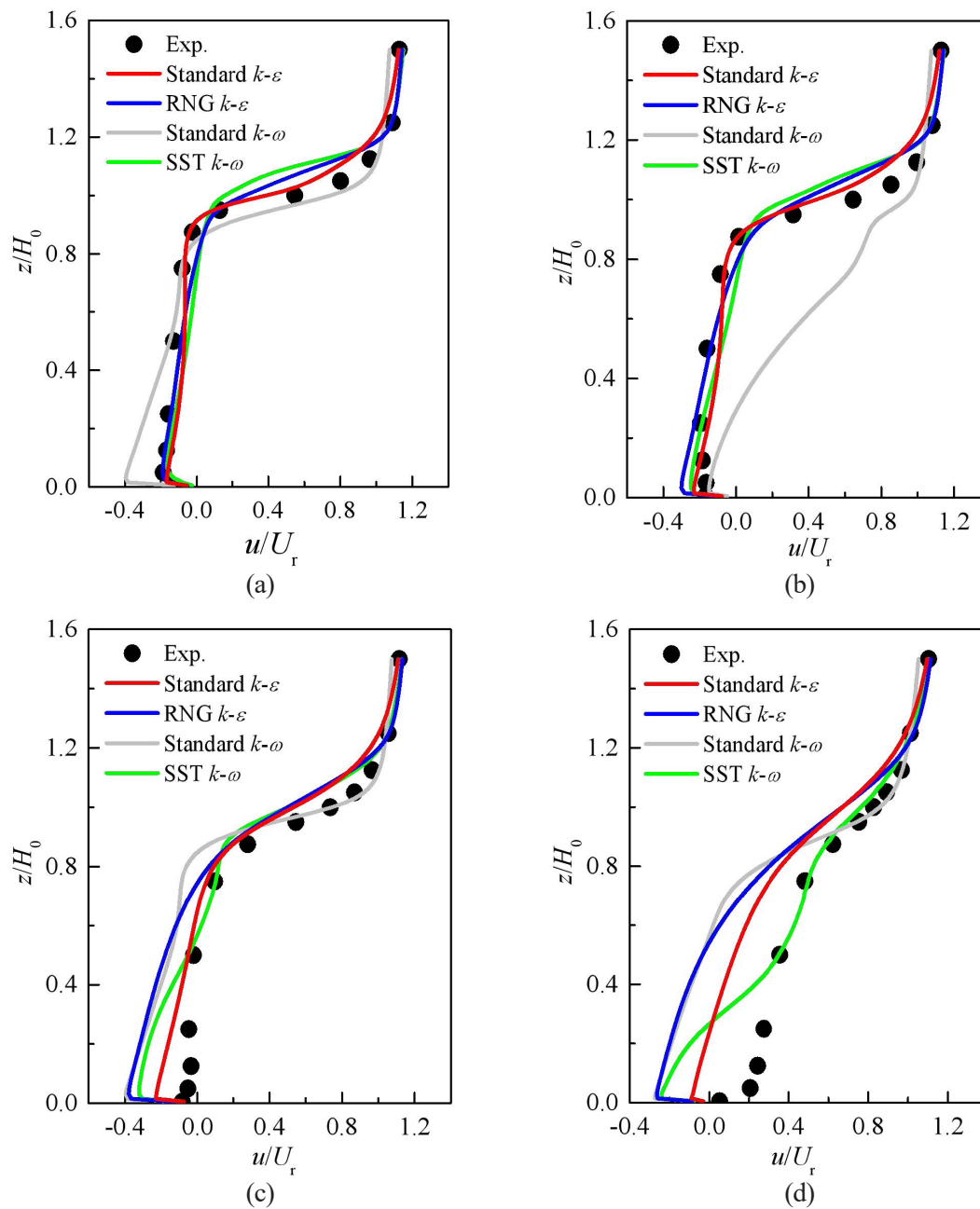
Fig. 3. Comparison of the velocity between CFD simulation results and experimental data: (a) line- x-H_0-0.125 , (b) line- x-H_0-0.25 , (c) line- x-H_0-0.5 , (d) line- x-H_0-1.0
