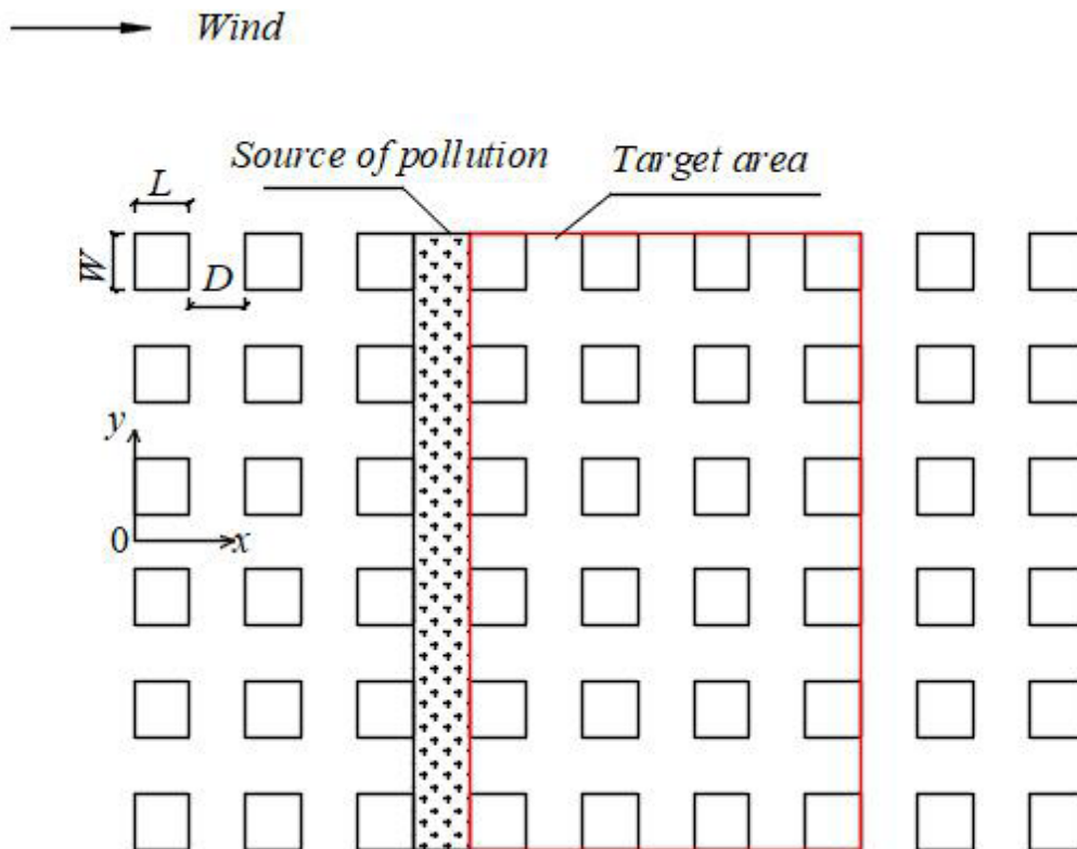
Fig. 6. Schematic of building layout
