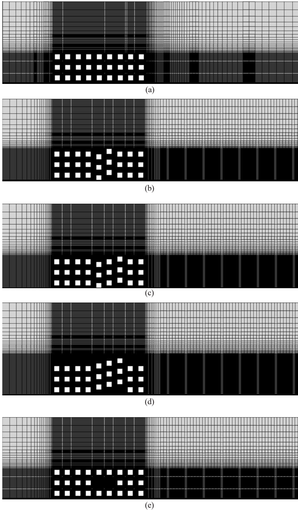
Fig. 8. Top view of the grid for five cases of building layouts: (a) case A (b) case B (c) case C (d) case D (e) case E
