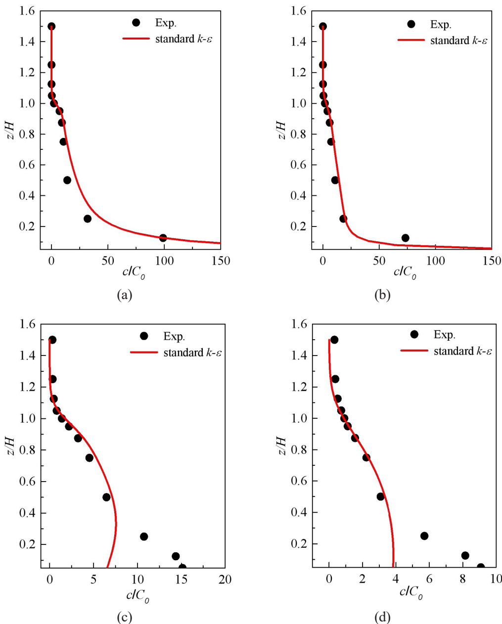
Fig. 5. Comparison of the concentration between CFD simulation results and experimental data: (a) line x-H_0-0.125 , (b) line x-H_0-0.25 , (c) line x-H_0-0.5 , (d) line x-H_0-1.0
