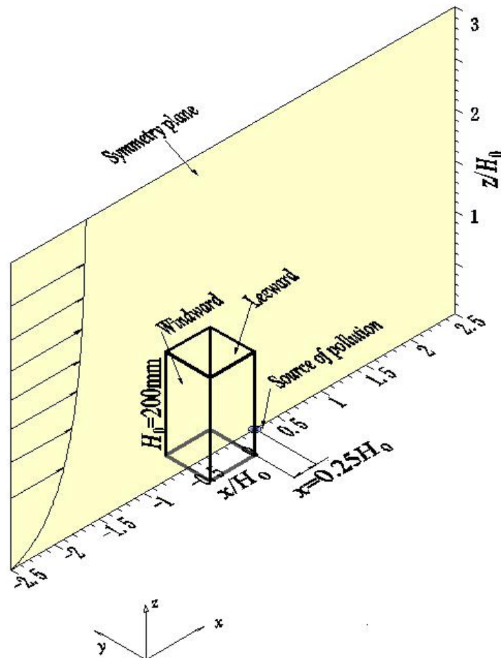
Fig. 1. Geometry of the building and point source [25]
