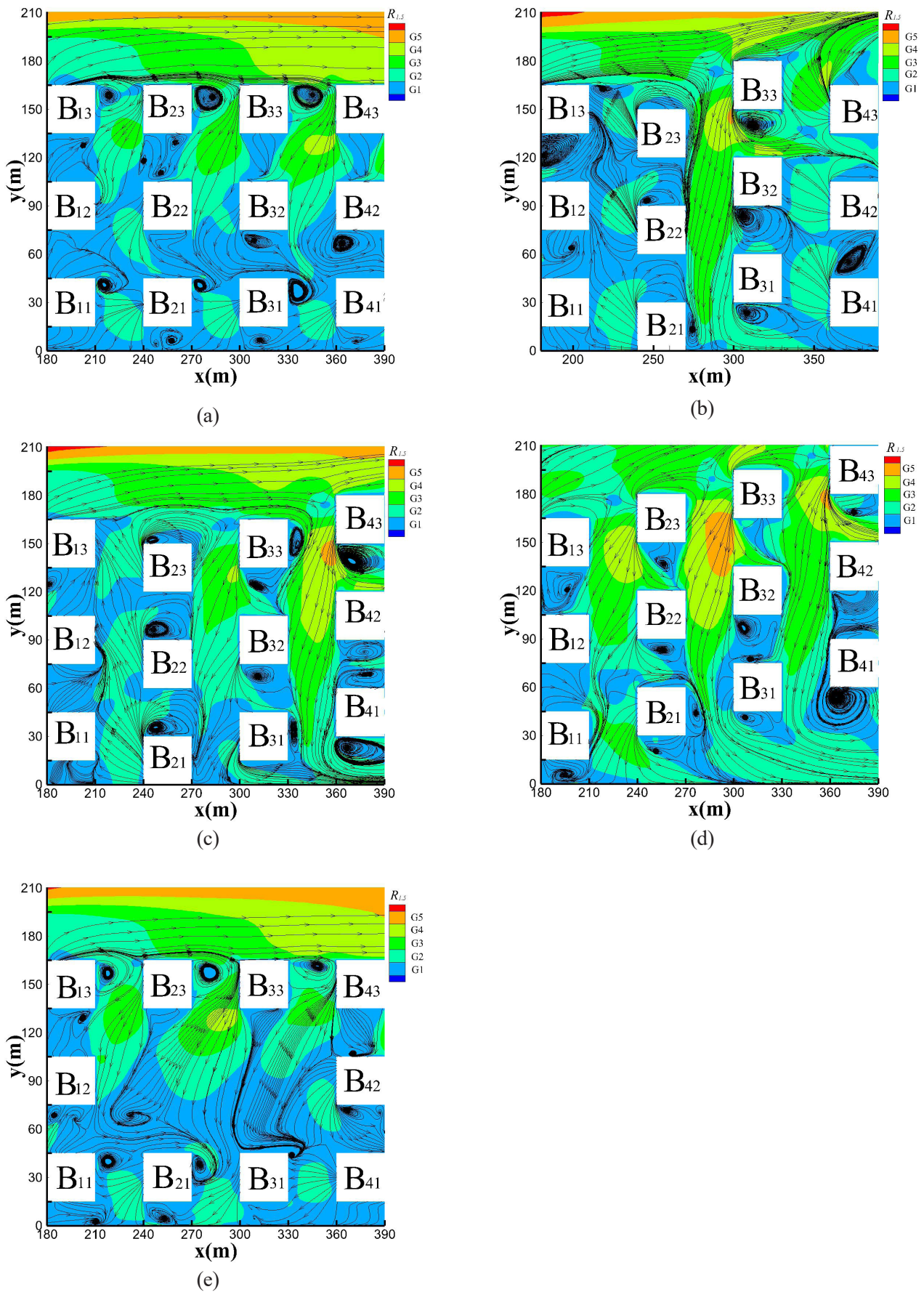
Fig. 9. Distribution of R_{1,5} and streamline at pedestrian level: (a) case A, (b) case B, (c) case C, (d) case D, (e) case E
