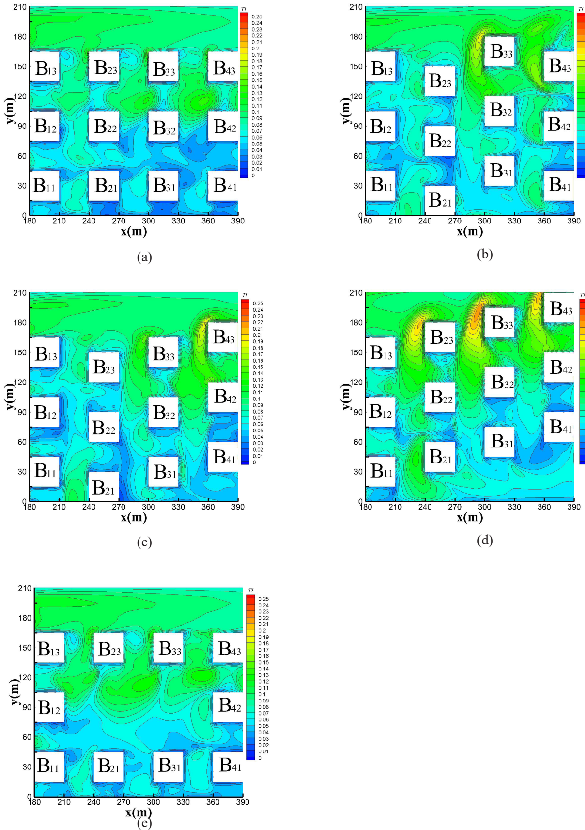
Fig. 11. Distribution of turbulent intensity at pedestrian level: (a) case A, (b) case B, (c) case C, (d) case D, (e) case E
