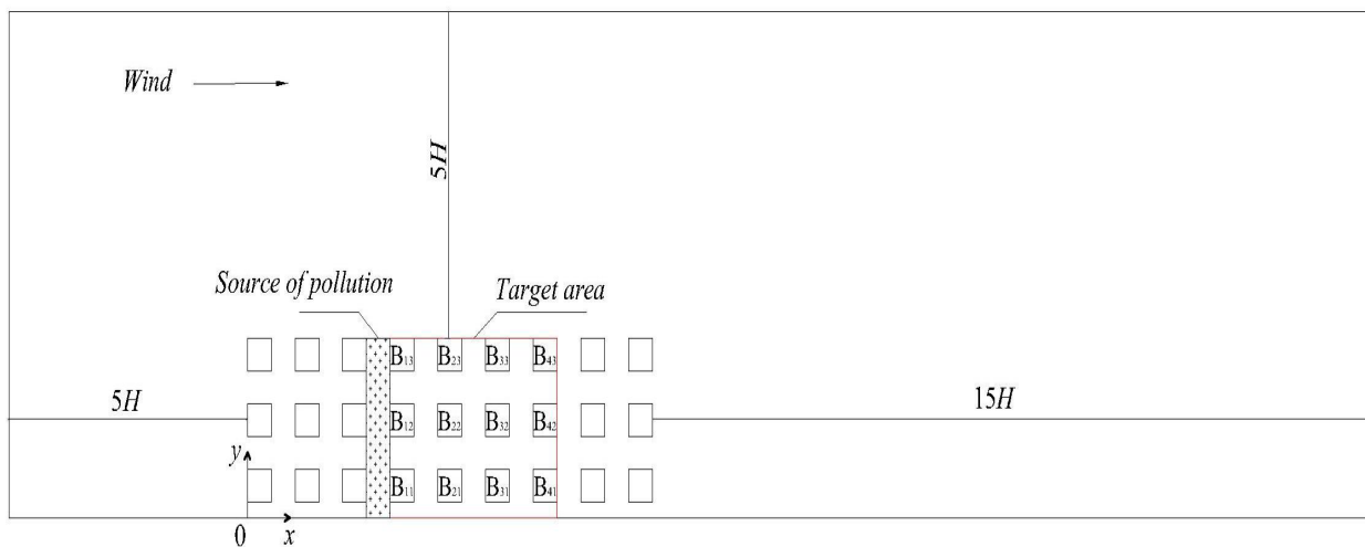
Fig. 7. Schematic of computational domain settings for building group
