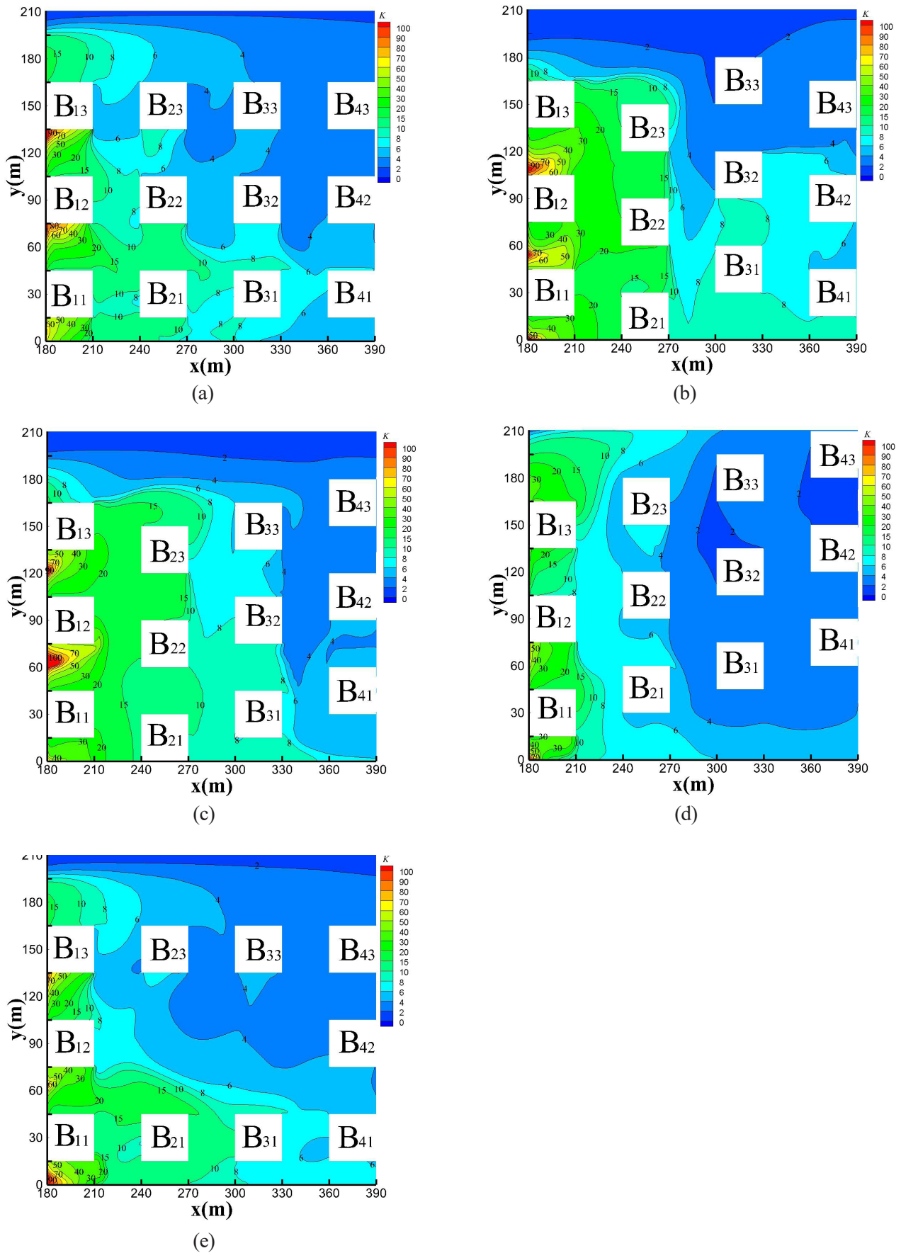
Fig. 10. Distribution of K at pedestrian level: (a) case A, (b) case B, (c) case C, (d) case D, (e) case E
