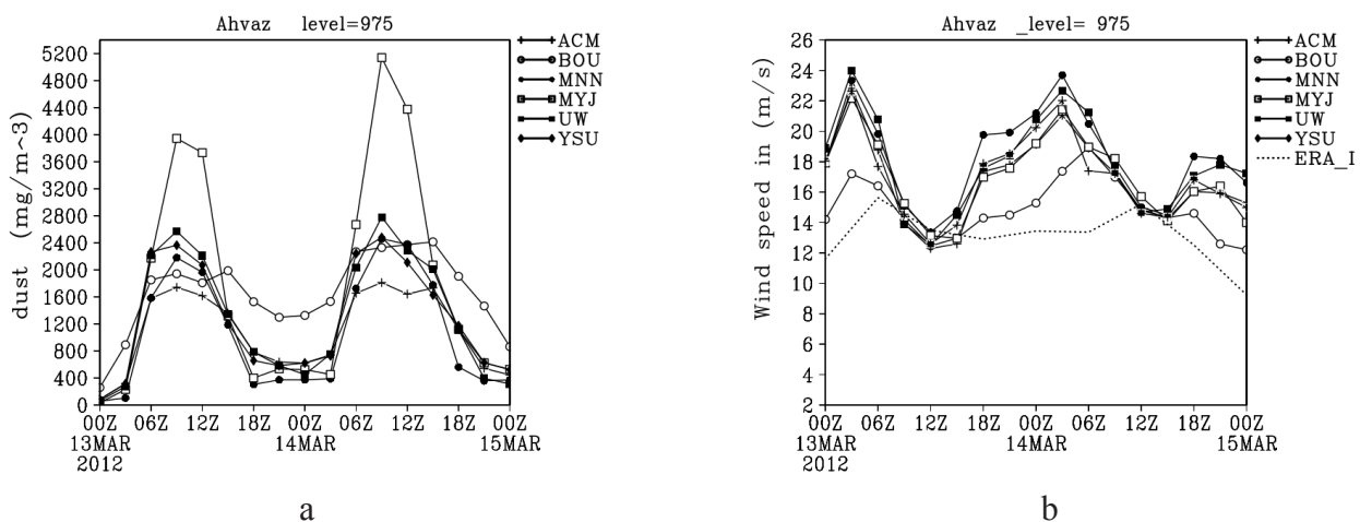
Fig. 9. The time series of a) PM_{10} \mu\text{g}/\text{m}^3 , b) wind speed (m/s) at 975hPa on March 13-14, 2012
