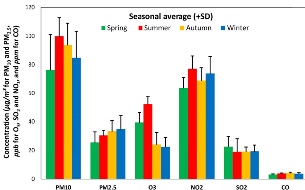
Fig. 2. Seasonal averages (+SD) of PM_{10} , PM_{2.5} , O_3 , NO_2 , SO_2 , and CO concentrations in Tehran during 2014-2018
